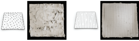
Figure 5: Left: surface sculpted with 100 toolpaths of 18 mm length in random direction, generated from 100 randomly sampled points; Right: the same surface sculpted with 15 parallel toolpaths across the whole width of the patch.
